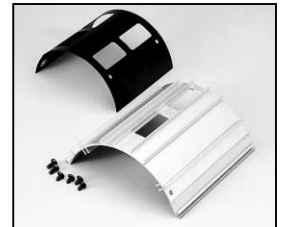
L4.77877.E Top cover cpl. Deckel kpl.
