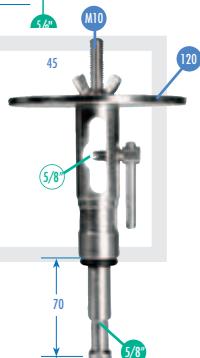
L2.89361.0 / LS.163-58F Spigot 1-1/8" + Bush 5/8"
