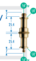
L2.76991.0 / LS.013 Adapter Spigot
