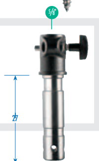
L2.89361.0 / LS.163-58F Spigot 1-1/8" + Bush 5/8"
