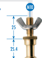
L2.88700.0 / LS.2064 Adapter 5/8" M-M10
