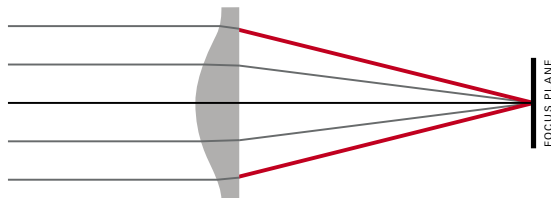
ASPHERICAL LENS
